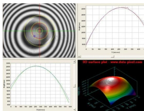
Interferometer testing
